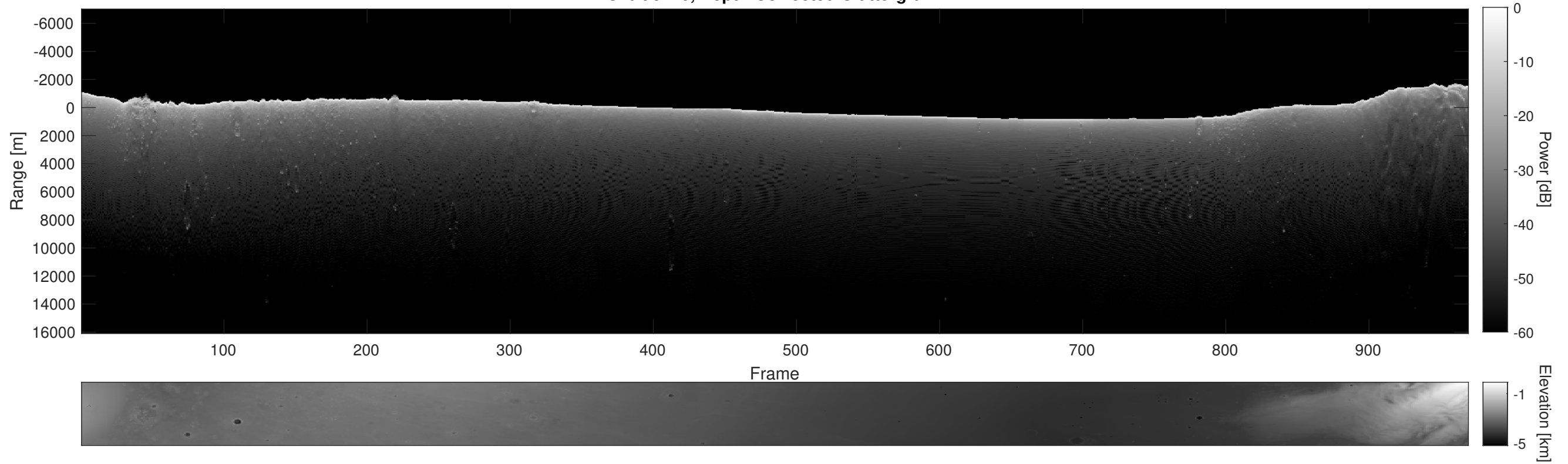
Orbit 9440, Depth-Corrected Cluttergram
