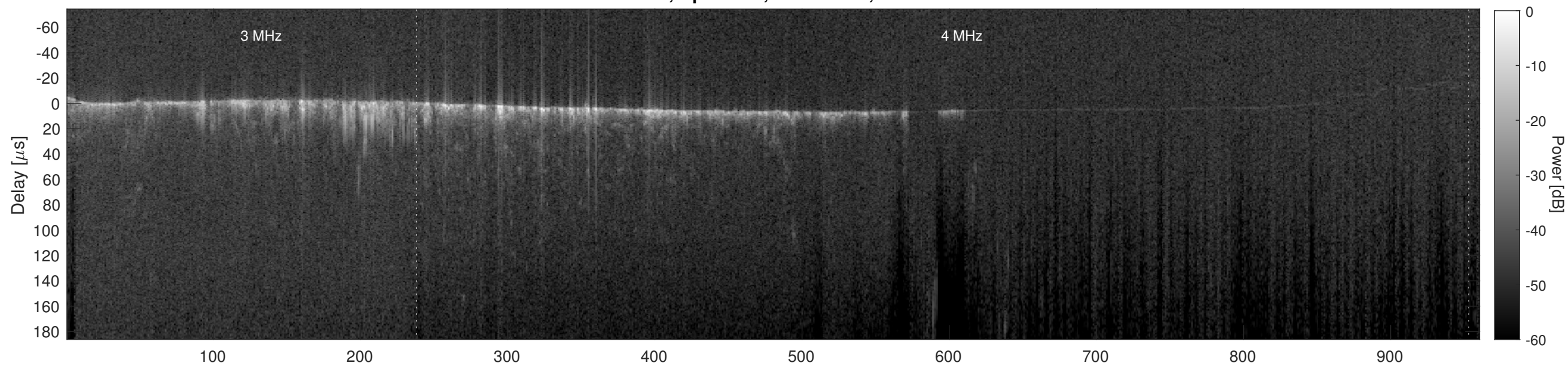
Orbit 9441, Cluttergram
