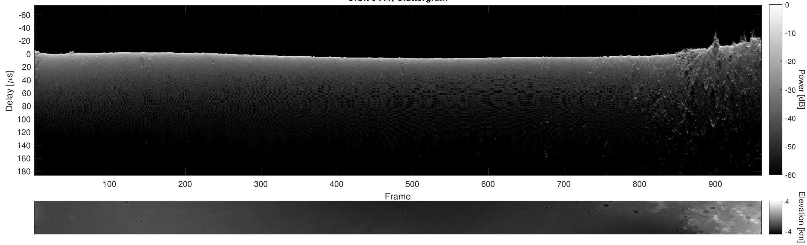
Orbit 9441, Cluttergram
