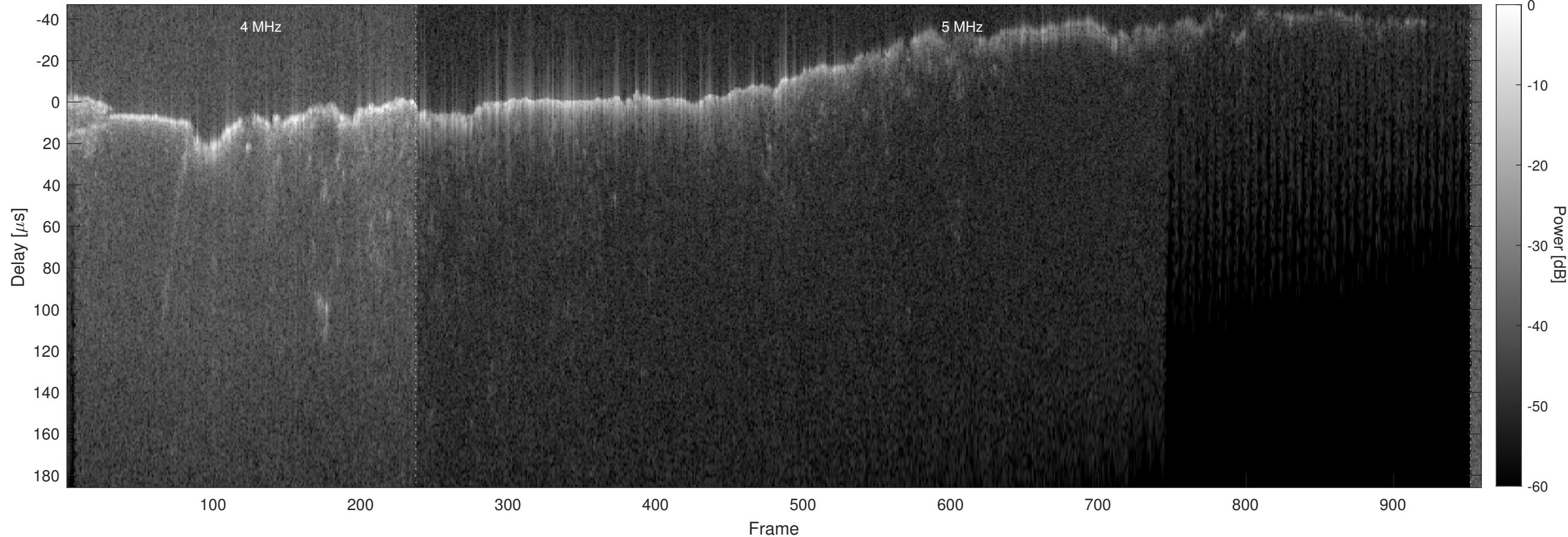
Orbit 9442, Chapman, No Window, Channel 2
