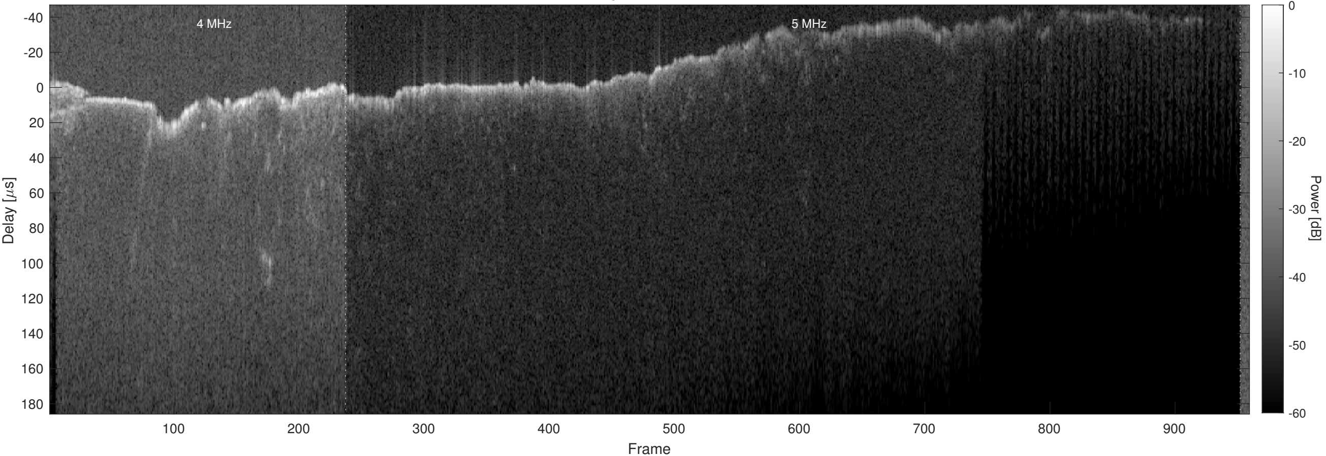
Orbit 9442, Chapman, Window, Channel 2
