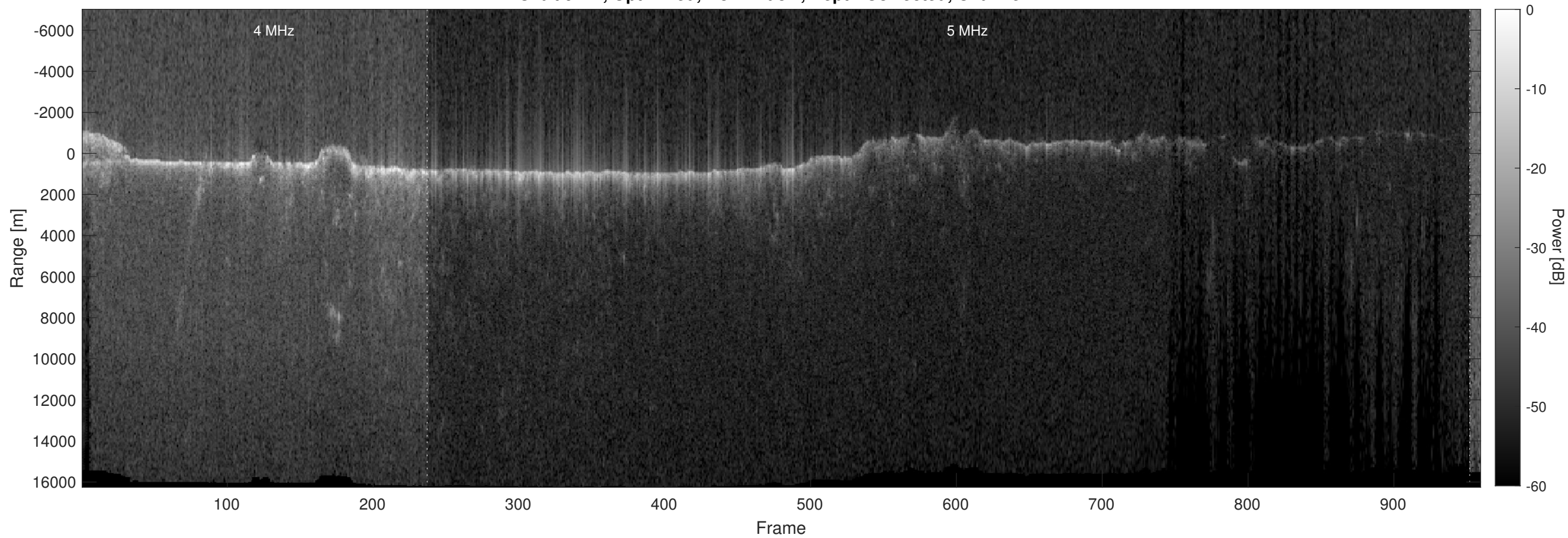
Orbit 9442, Optimized, No Window, Depth-Corrected, Channel 2
