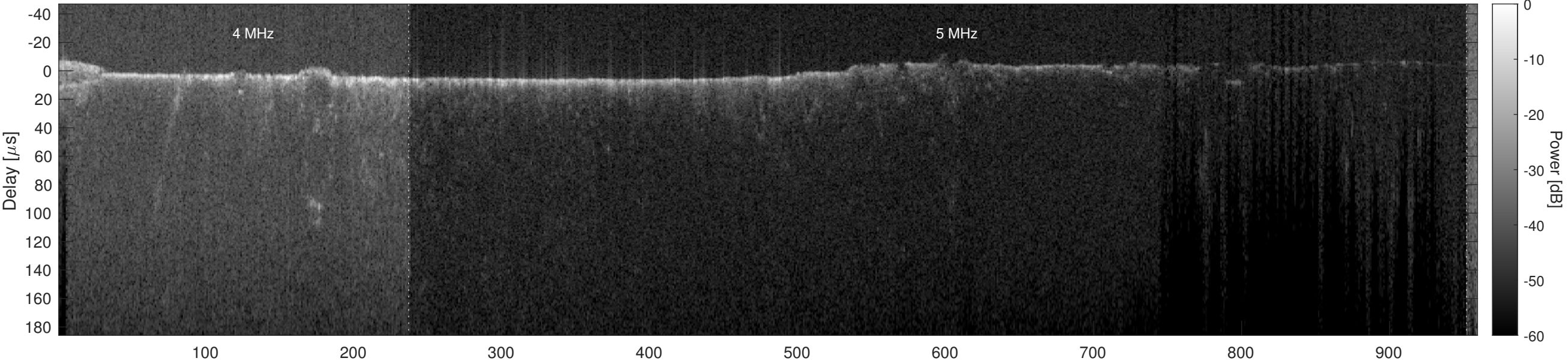
Orbit 9442, Optimized, Window, Channel 2
