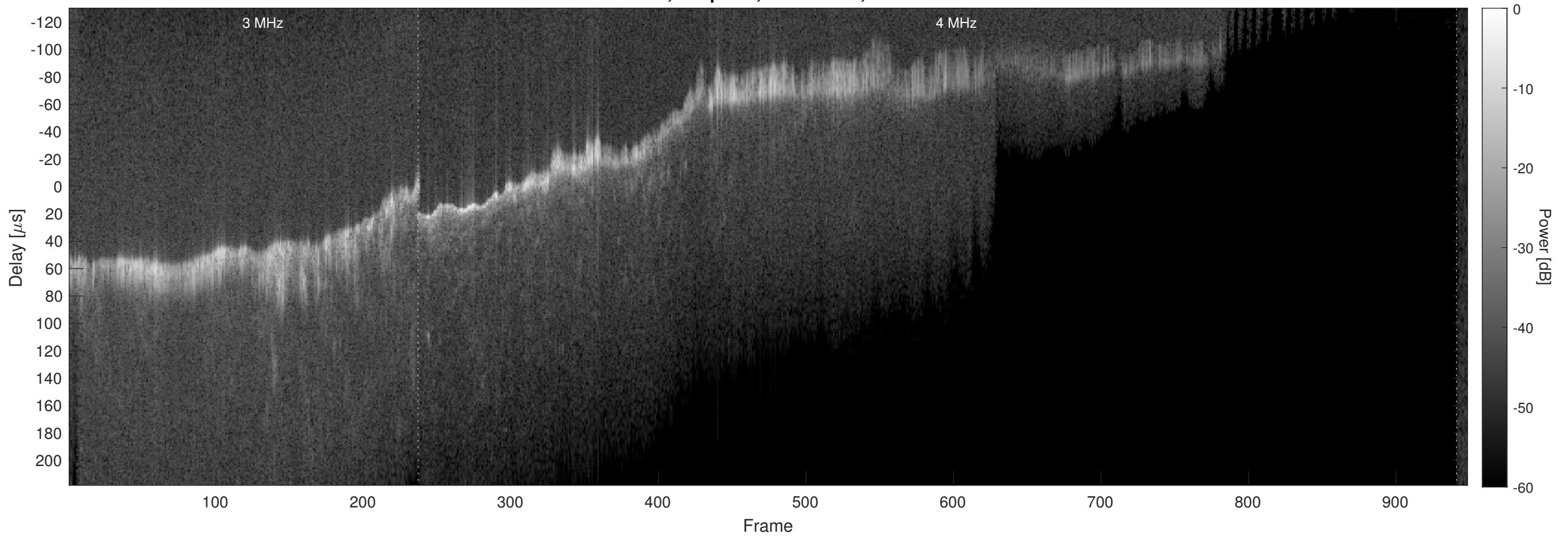
Orbit 9443, Chapman, No Window, Channel 2
