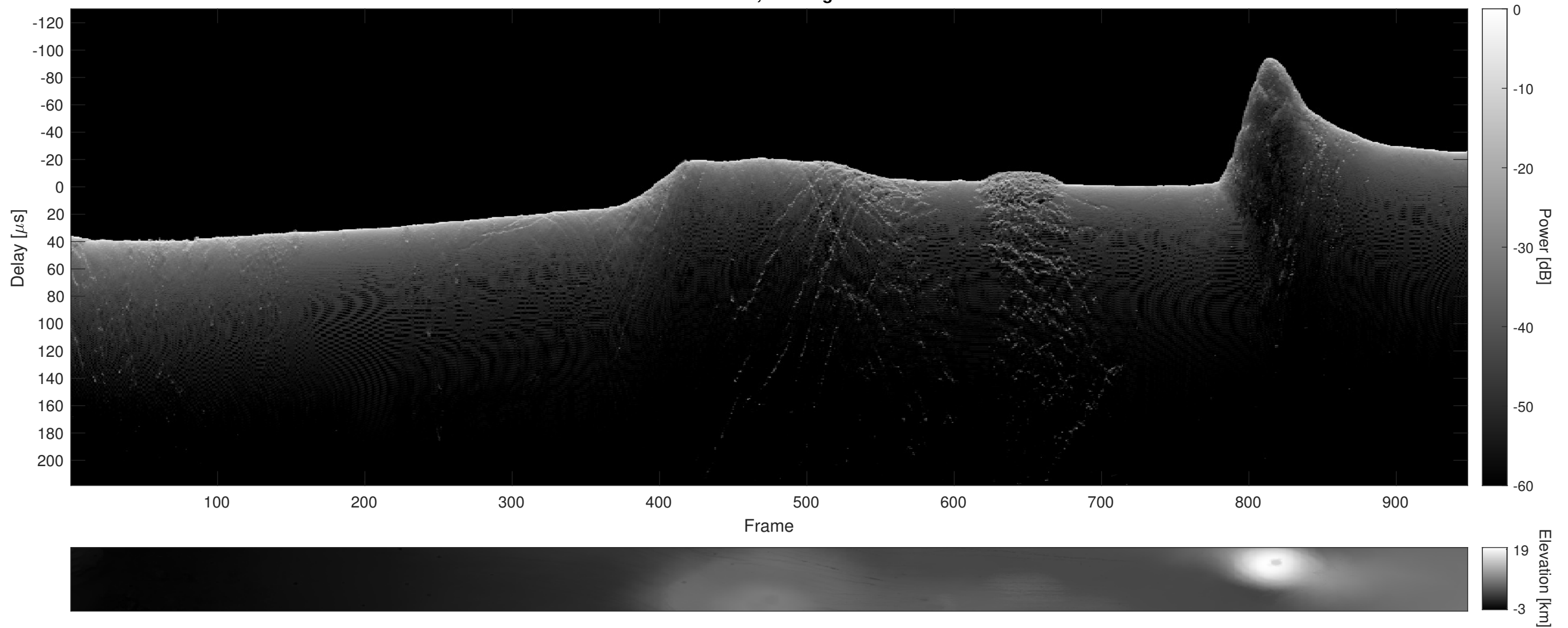
Orbit 9443, Cluttergram
