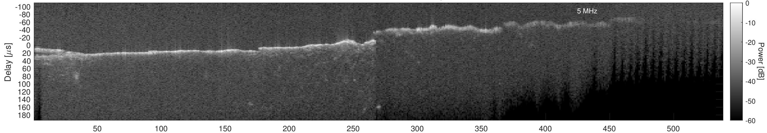
Orbit 9445, Window, Channel 2, Optimized
