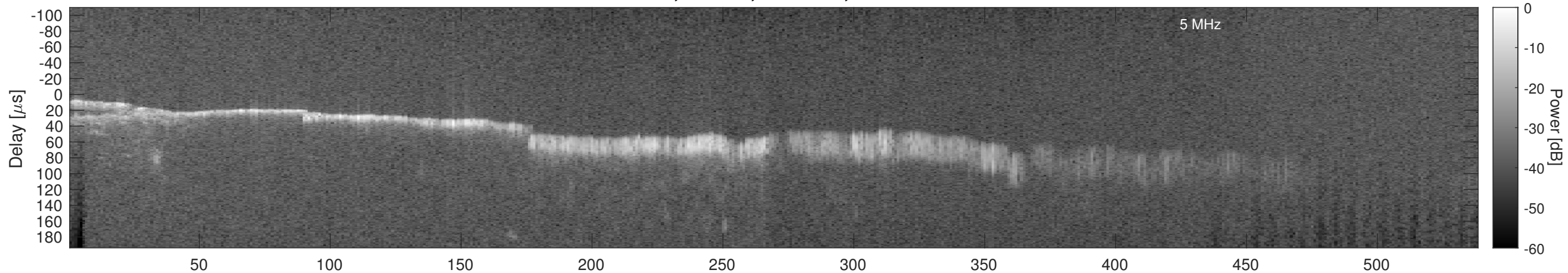
Orbit 9445, Window, Channel 2, Chapman
