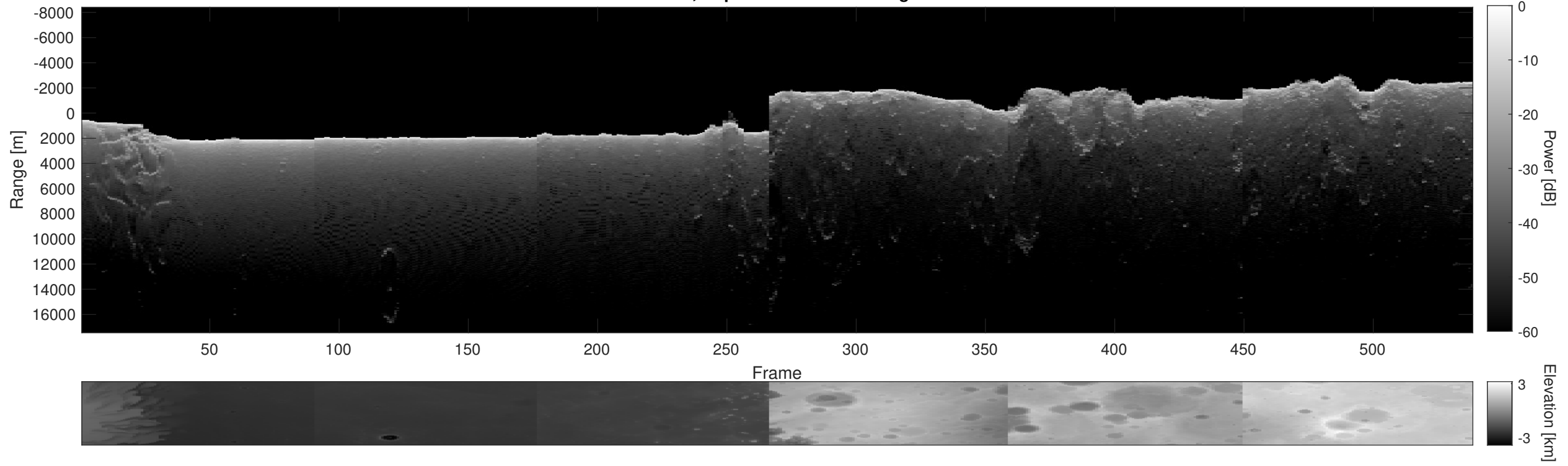
Orbit 9445, Depth-Corrected Cluttergram
