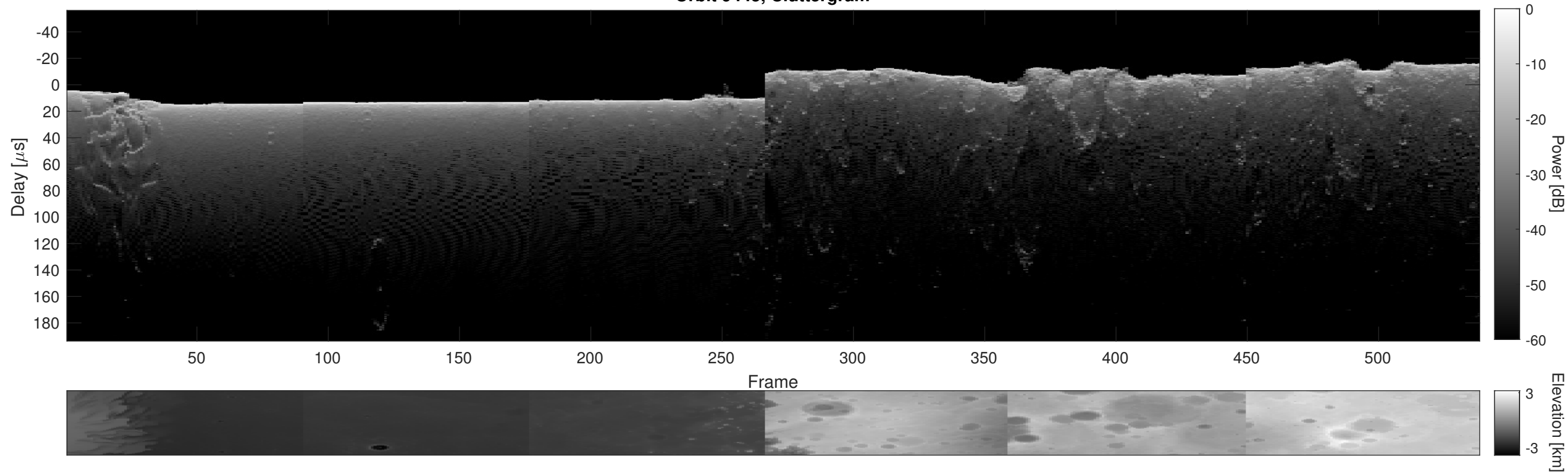
Orbit 9445, Cluttergram
