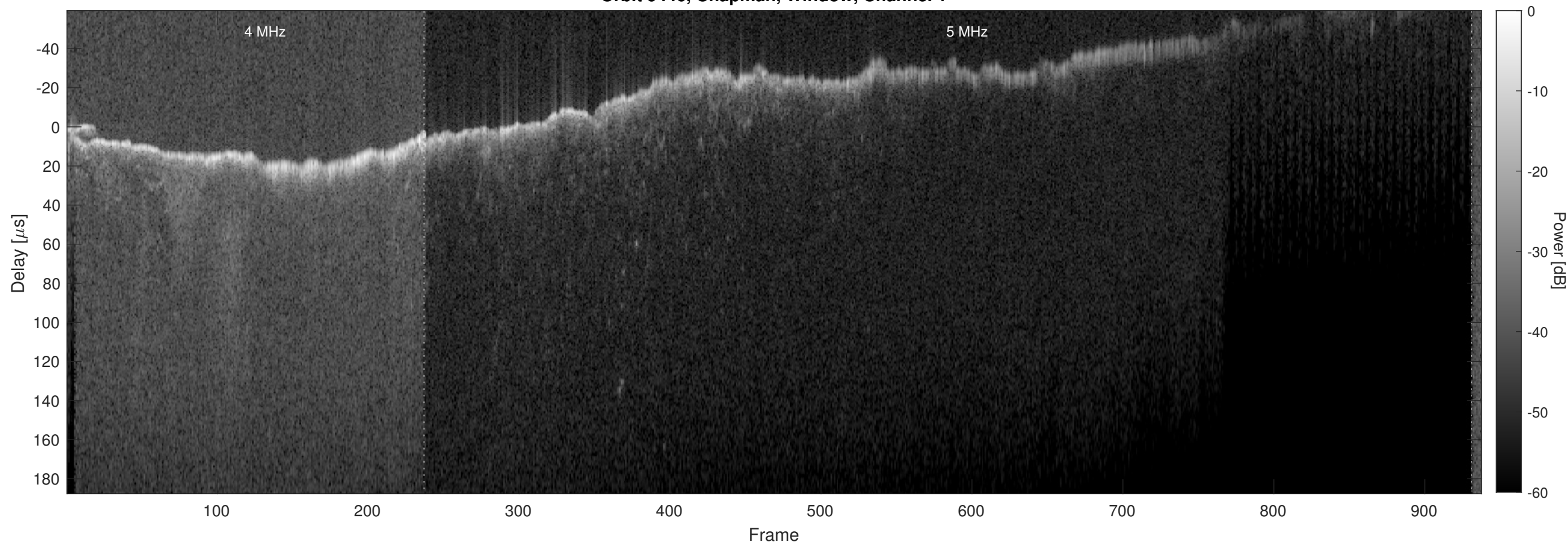
Orbit 9446, Chapman, Window, Channel 2
