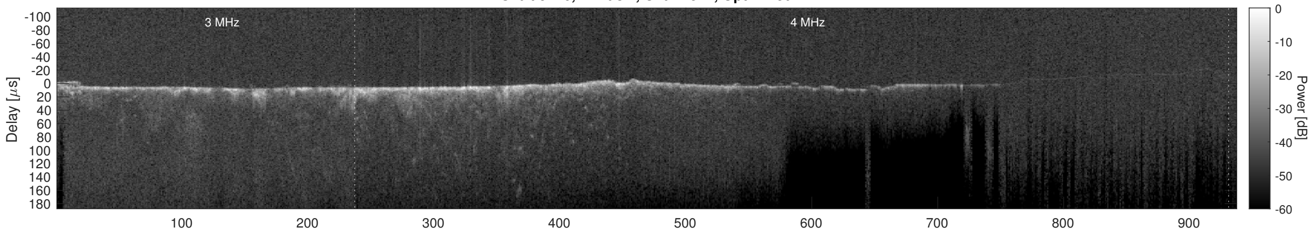
Orbit 9446, Cluttergram
