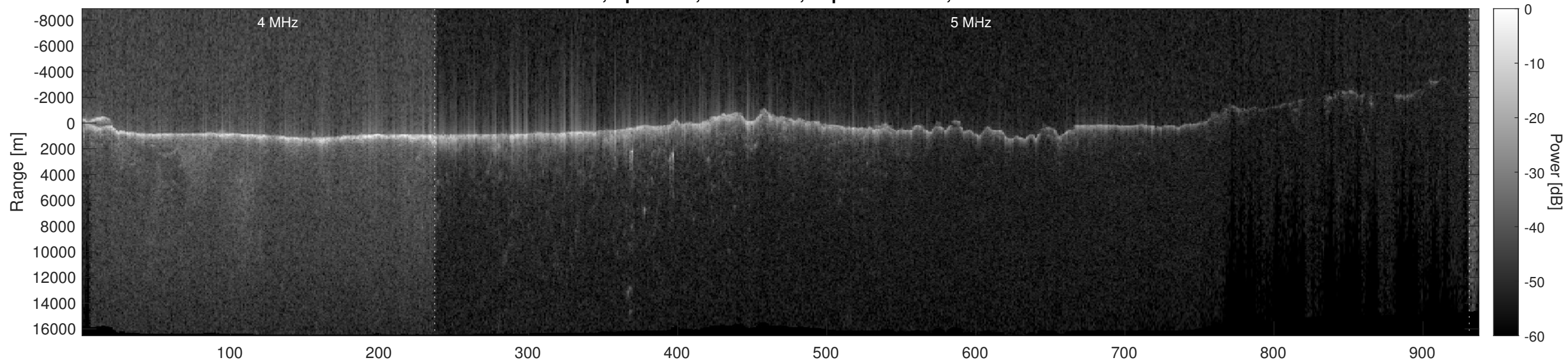
Orbit 9446, Optimized, No Window, Depth-Corrected, Channel 2
