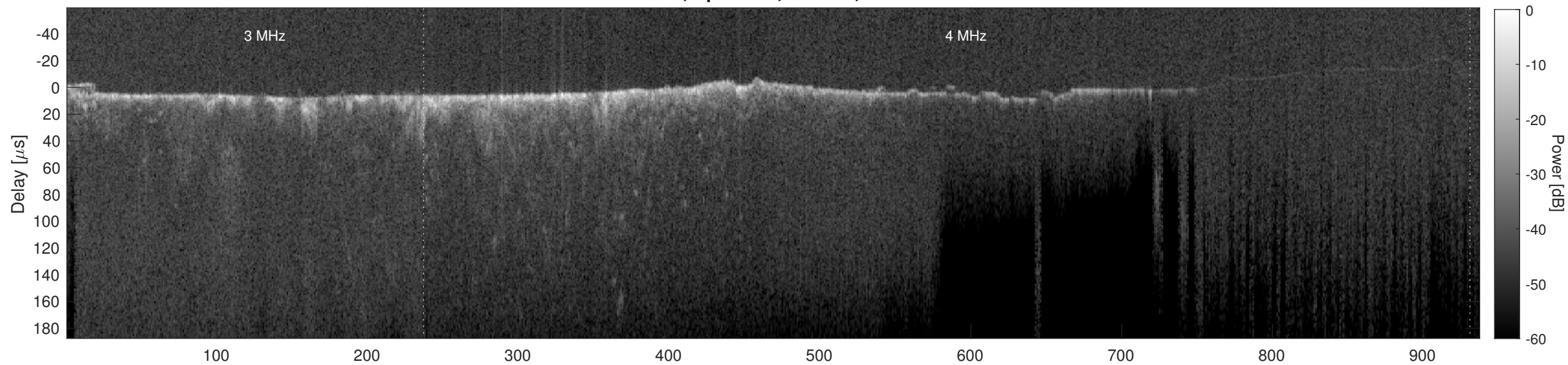
Orbit 9446, Cluttergram
