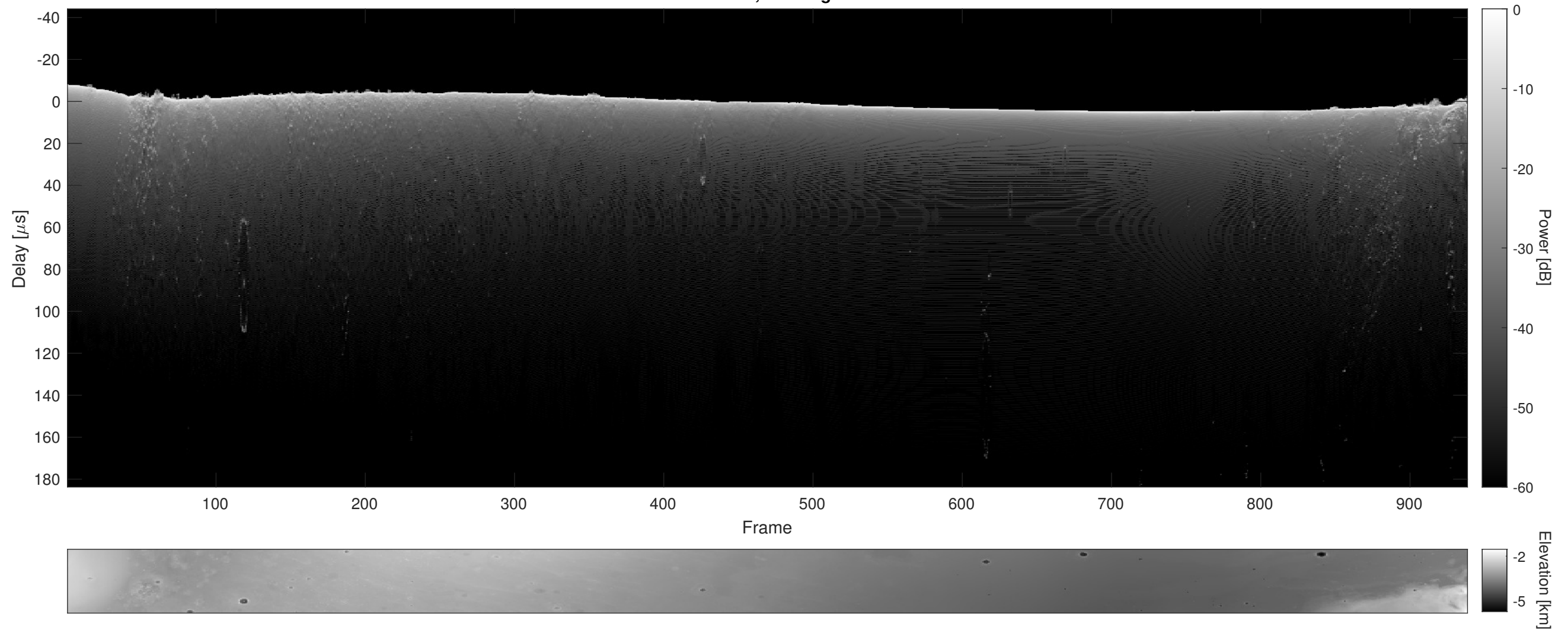
Orbit 9447, Cluttergram
