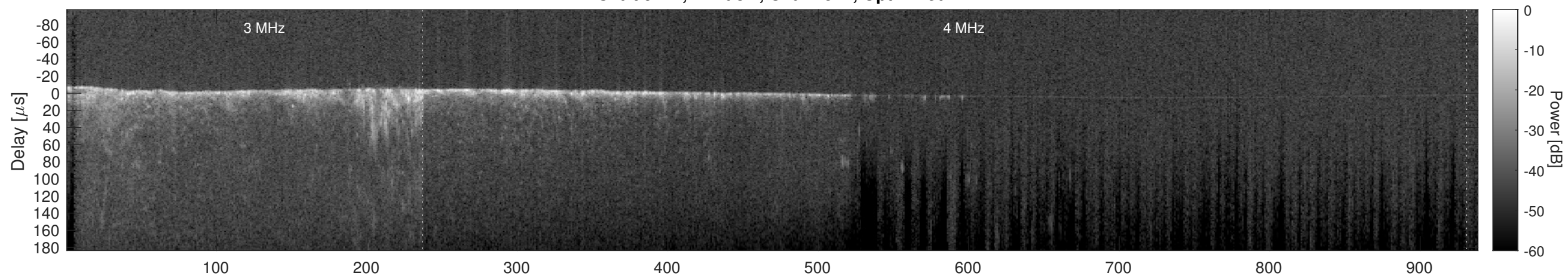
Orbit 9447, Cluttergram
