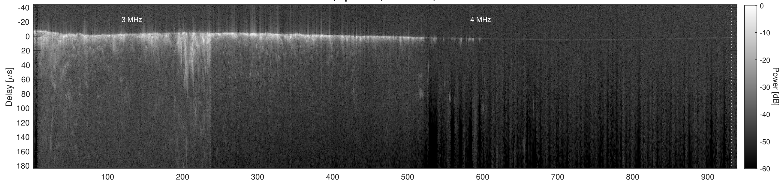
Orbit 9447, Cluttergram
