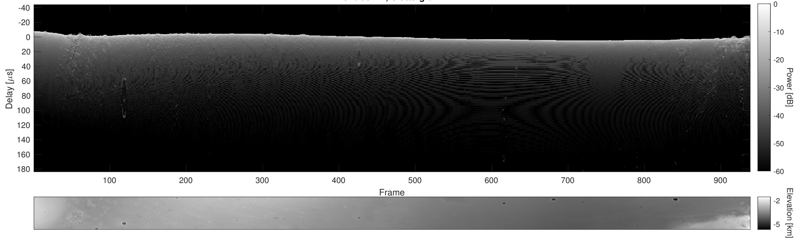
Orbit 9447, Cluttergram
