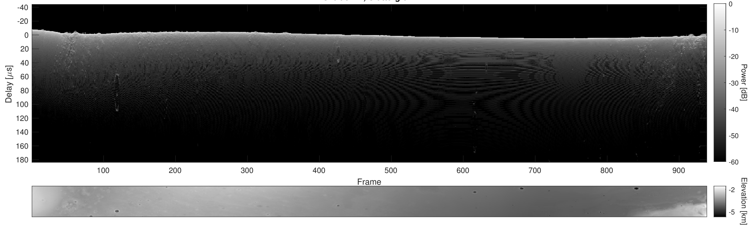
Orbit 9447, Cluttergram
