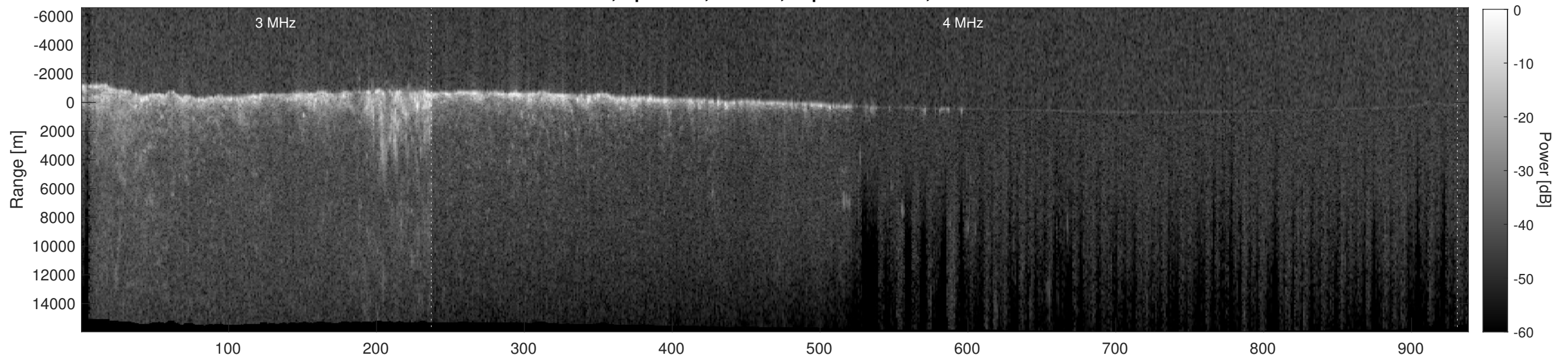
Orbit 9447, Depth-Corrected Cluttergram
