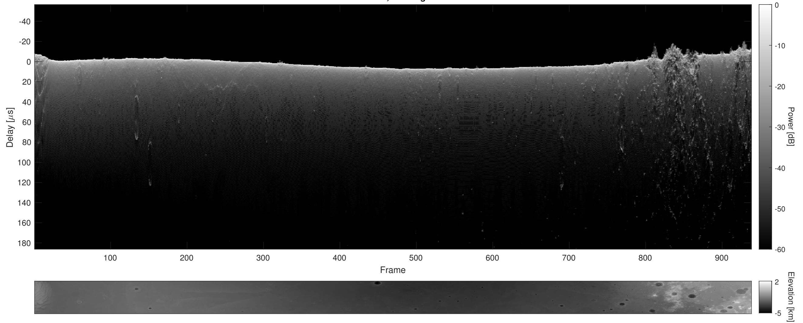
Orbit 9448, Cluttergram
