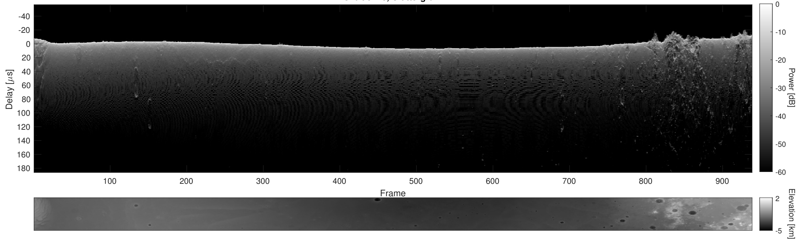
Orbit 9448, Cluttergram
