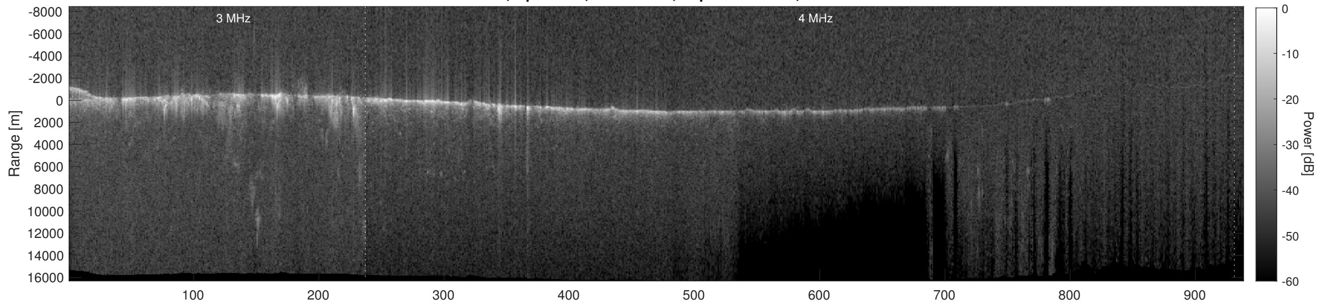
Orbit 9448, Depth-Corrected Cluttergram
