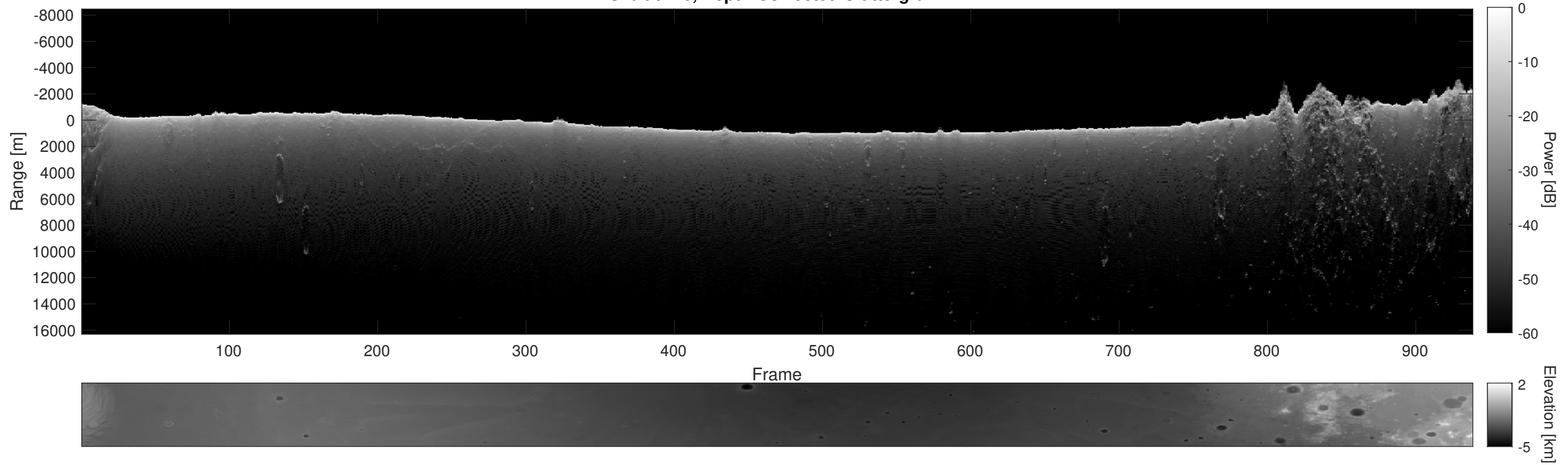
Orbit 9448, Depth-Corrected Cluttergram
