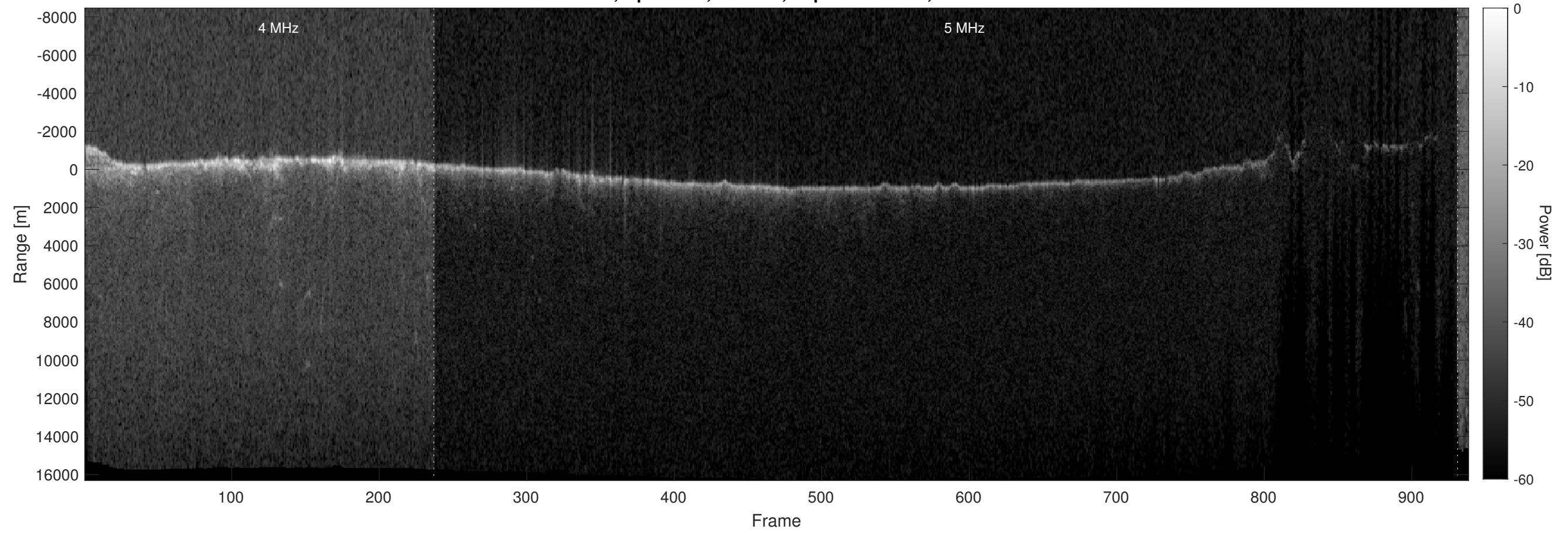
Orbit 9448, Optimized, Window, Depth-Corrected, Channel 2
