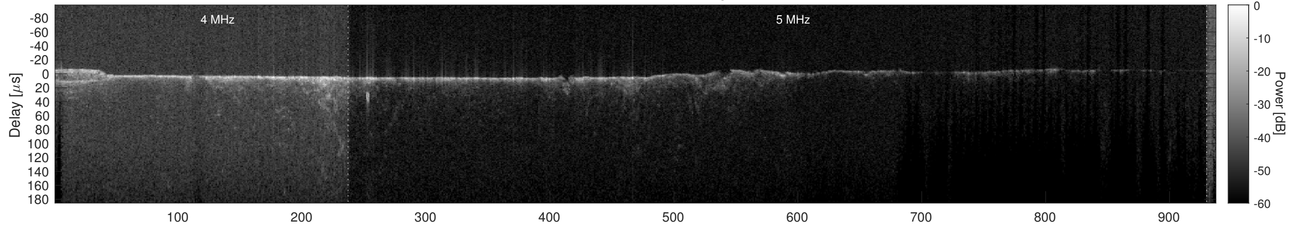
Orbit 9449, Cluttergram
