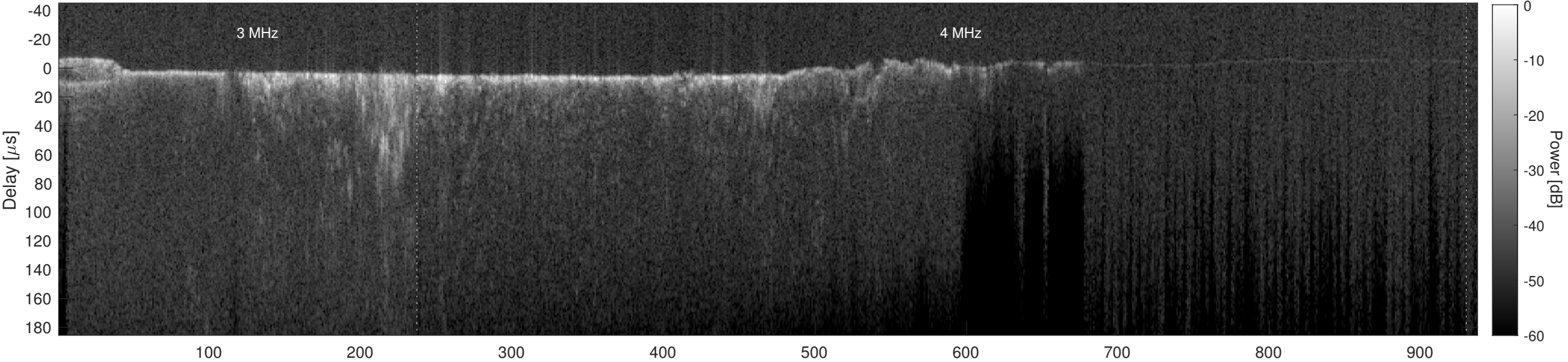
Orbit 9449, Cluttergram
