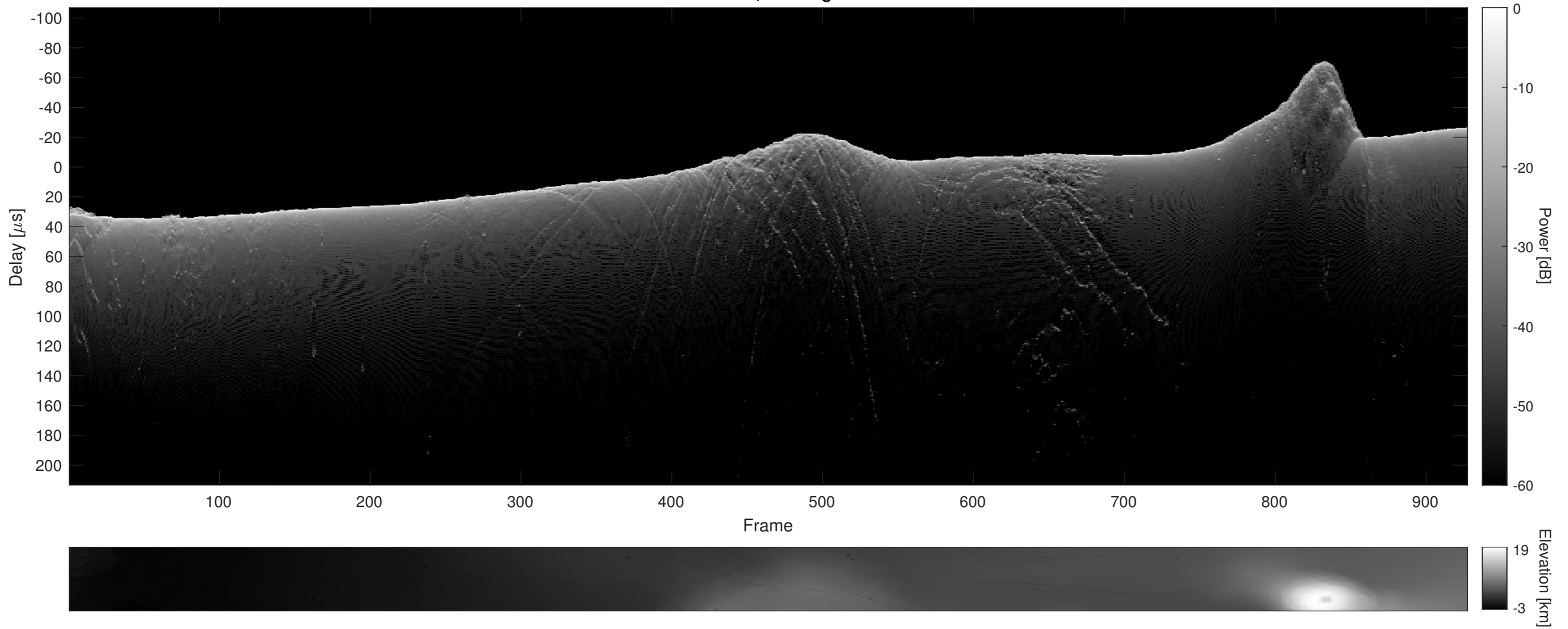
Orbit 9450, Cluttergram
