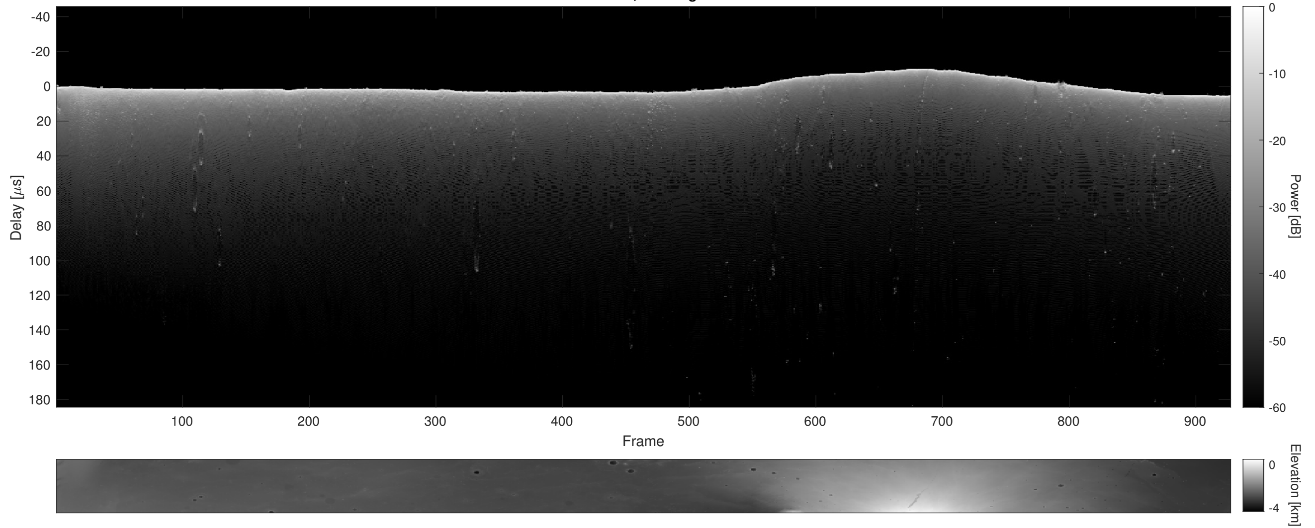
Orbit 9451, Cluttergram
