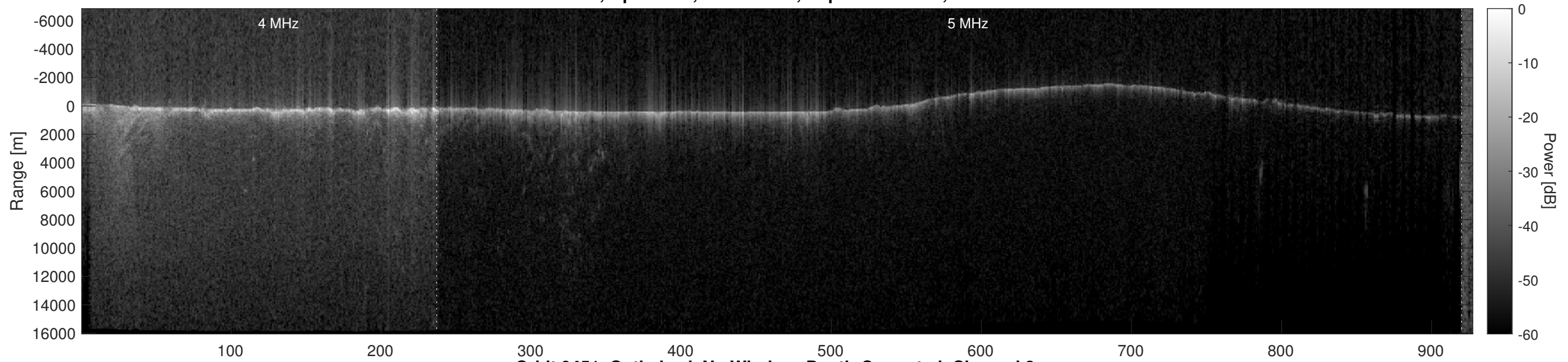
Orbit 9451, Optimized, No Window, Depth-Corrected, Channel 2
