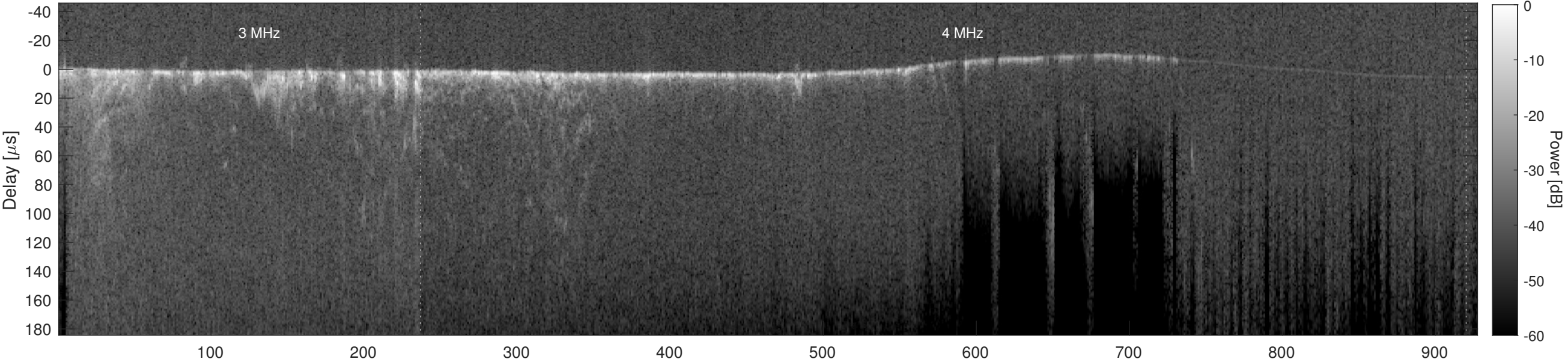
Orbit 9451, Cluttergram
