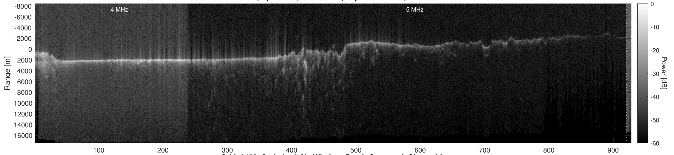
Orbit 9452, Optimized, No Window, Depth-Corrected, Channel 2
