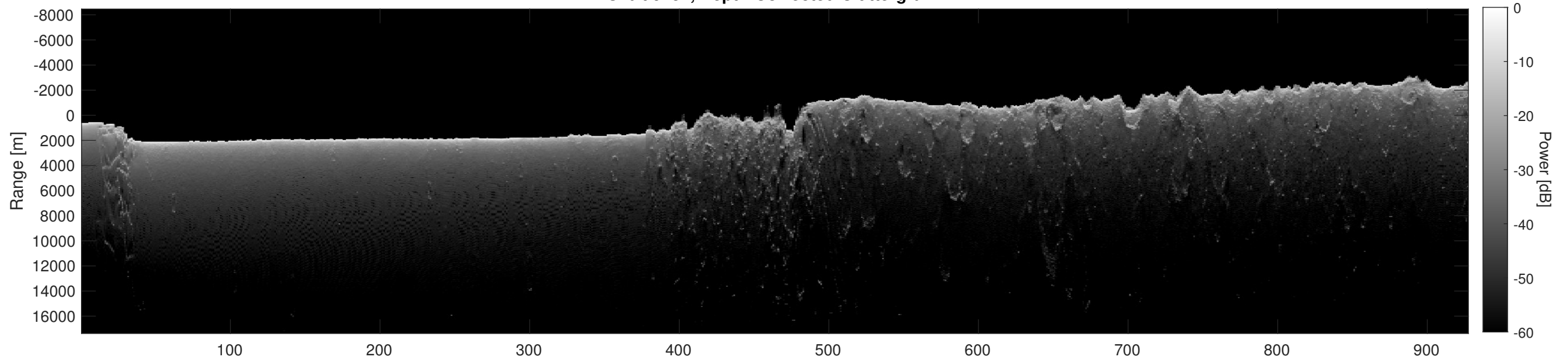
Orbit 9452, Depth-Corrected Cluttergram
