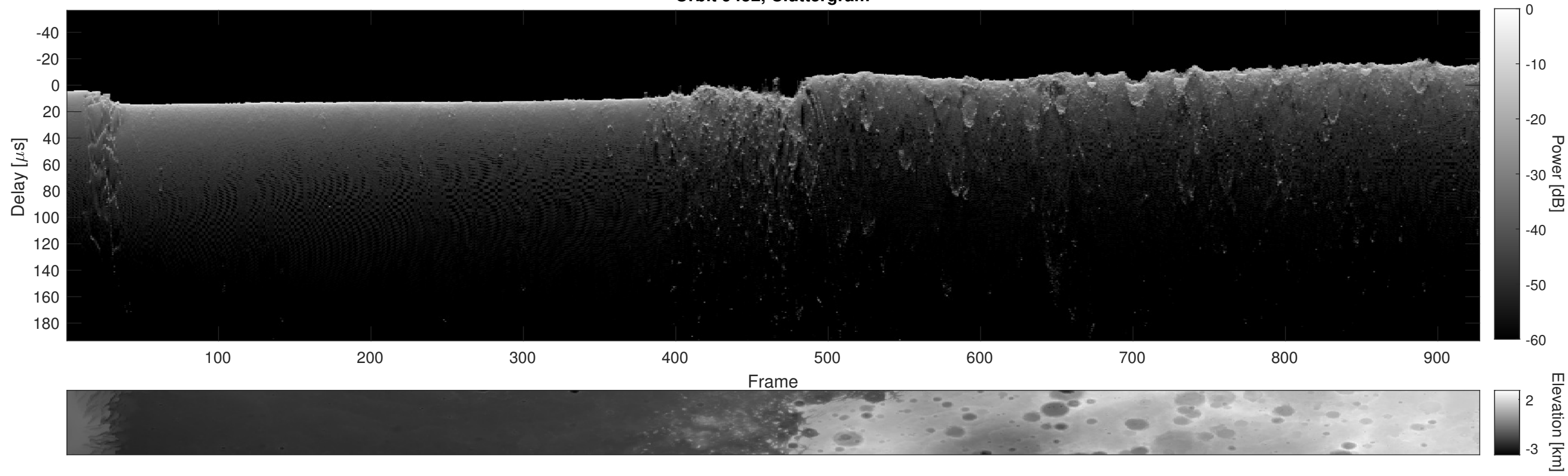
Orbit 9452, Cluttergram
