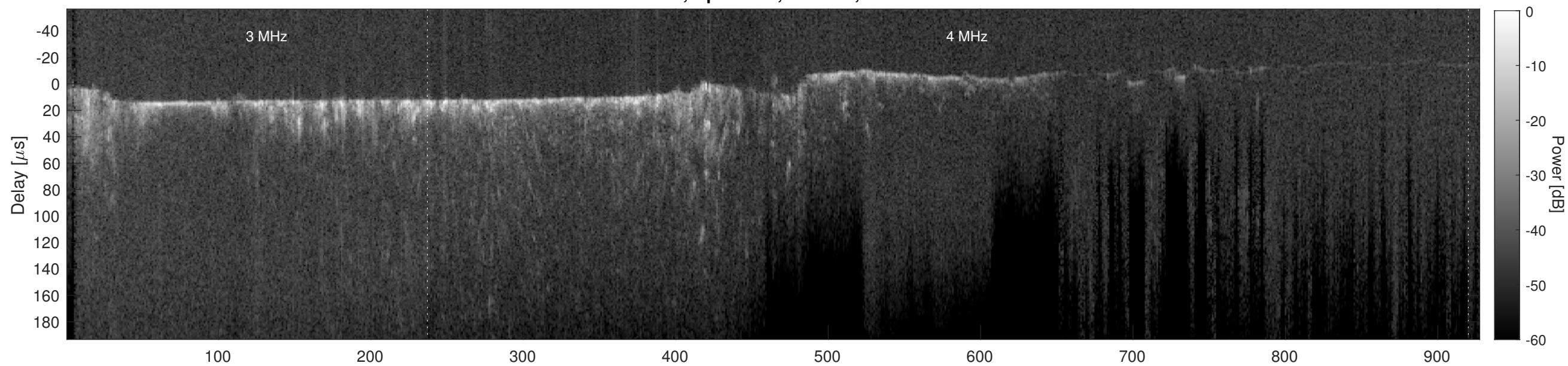
Orbit 9452, Cluttergram
