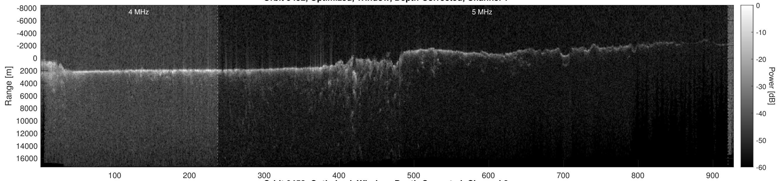
Orbit 9452, Optimized, Window, Depth-Corrected, Channel 2
