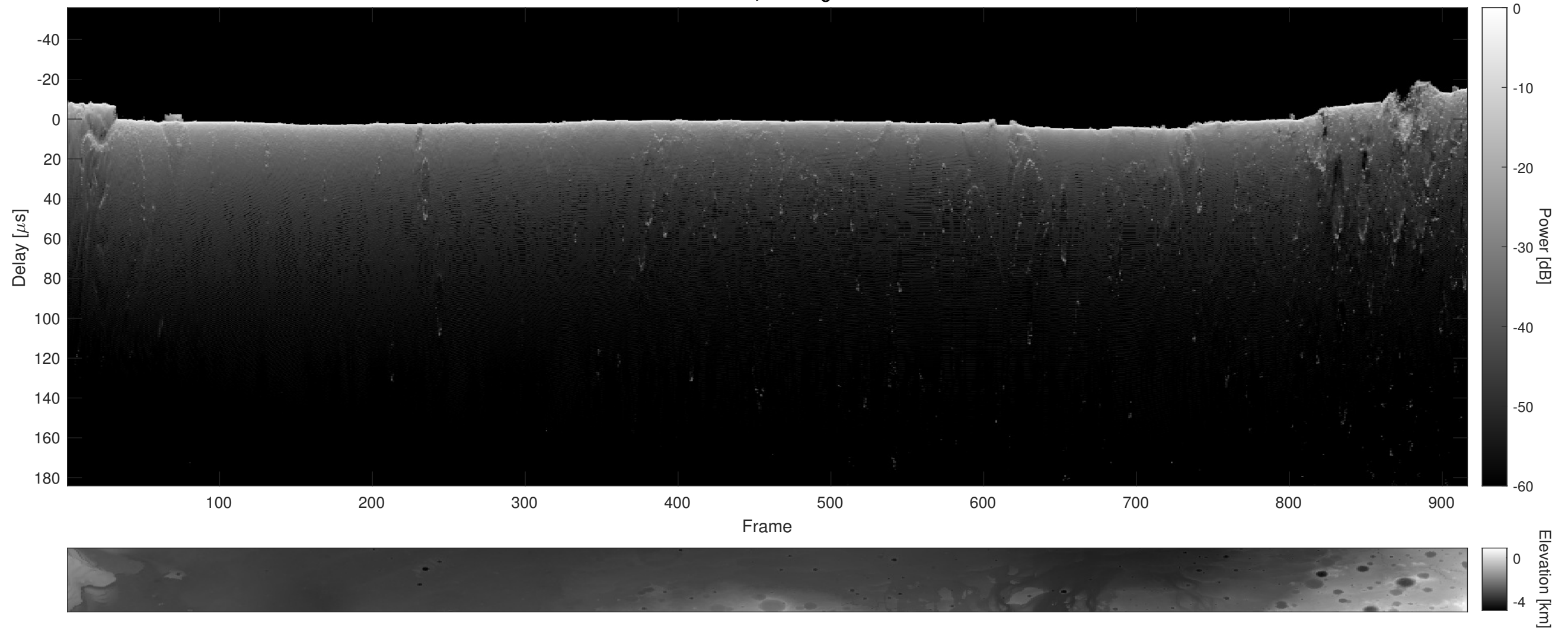
Orbit 9453, Cluttergram
