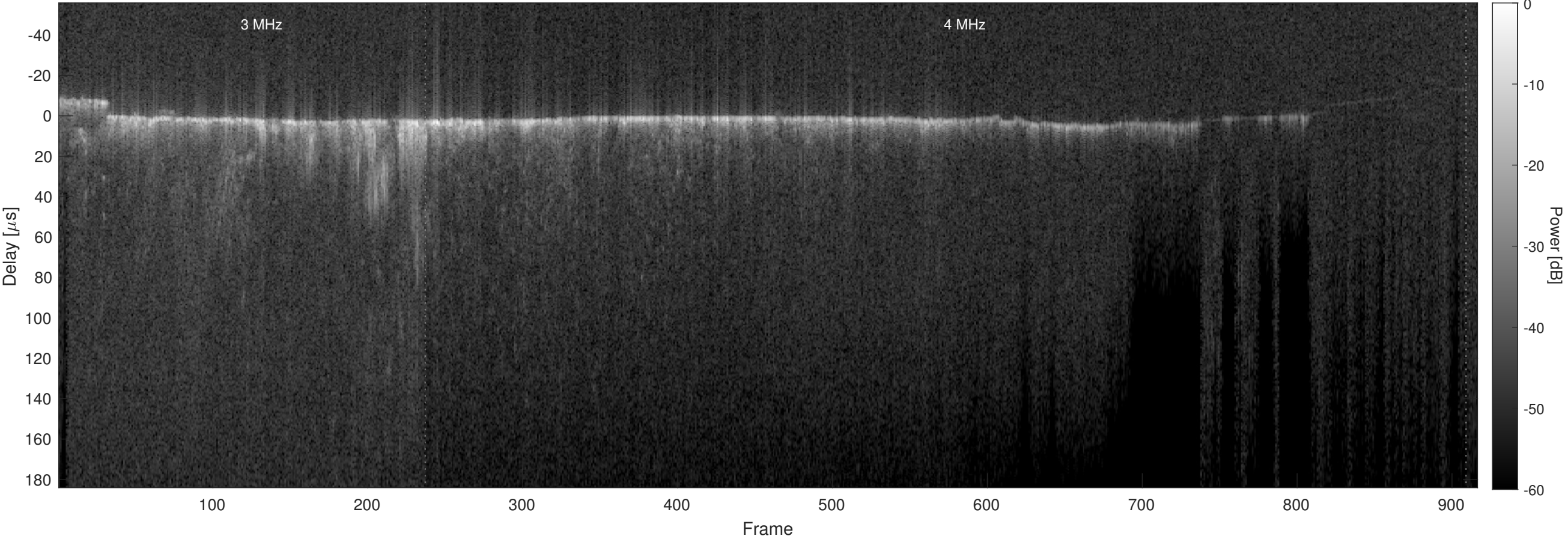
Orbit 9453, Optimized, No Window, Channel 2
