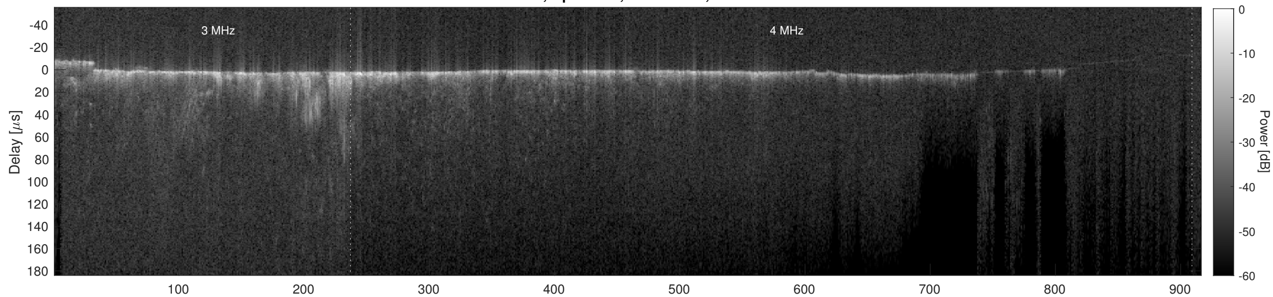
Orbit 9453, Cluttergram
