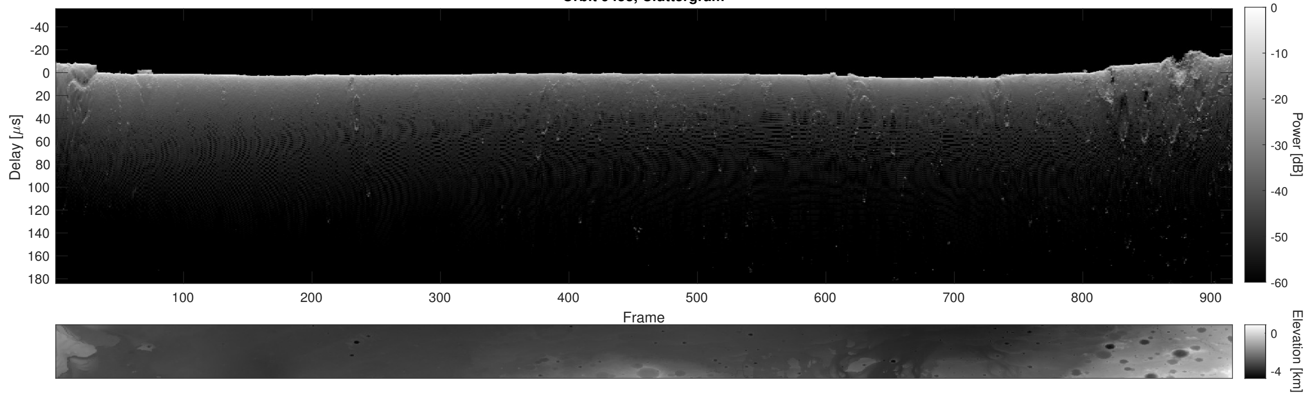
Orbit 9453, Cluttergram
