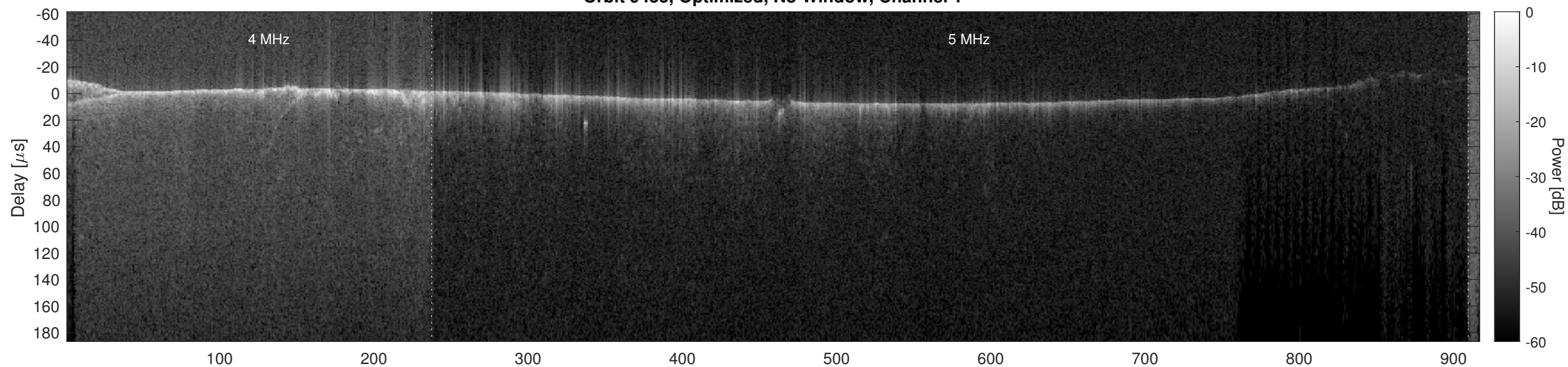
Orbit 9455, Optimized, No Window, Channel 2
