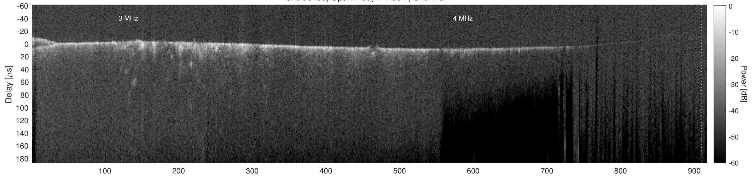
Orbit 9455, Cluttergram
