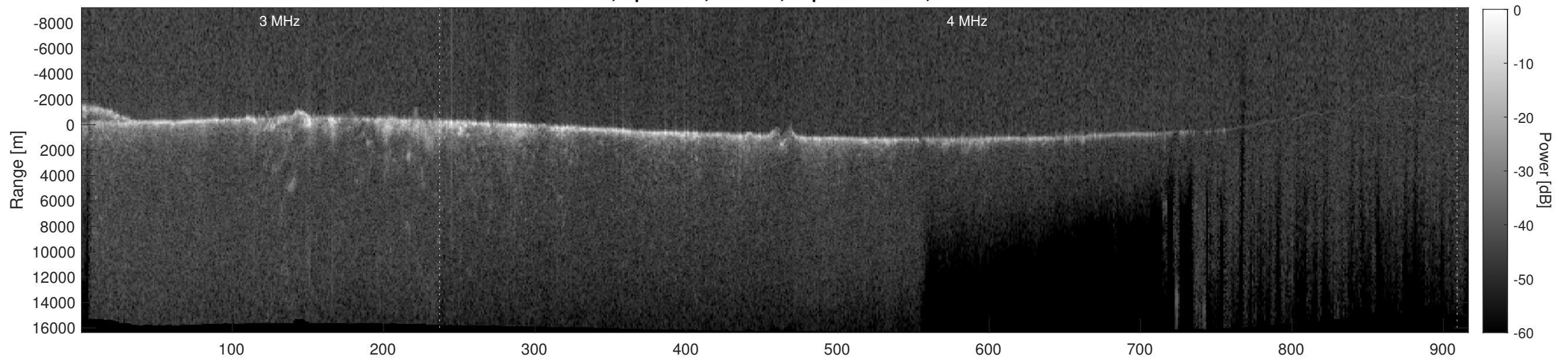
Orbit 9455, Depth-Corrected Cluttergram
