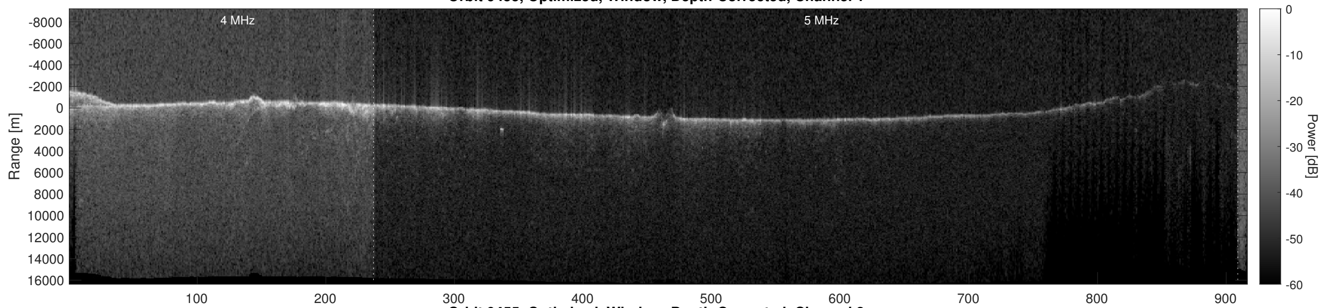
Orbit 9455, Optimized, Window, Depth-Corrected, Channel 2
