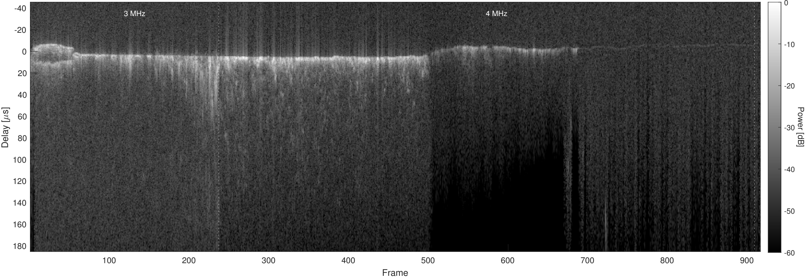
Orbit 9456, Optimized, No Window, Channel 2
