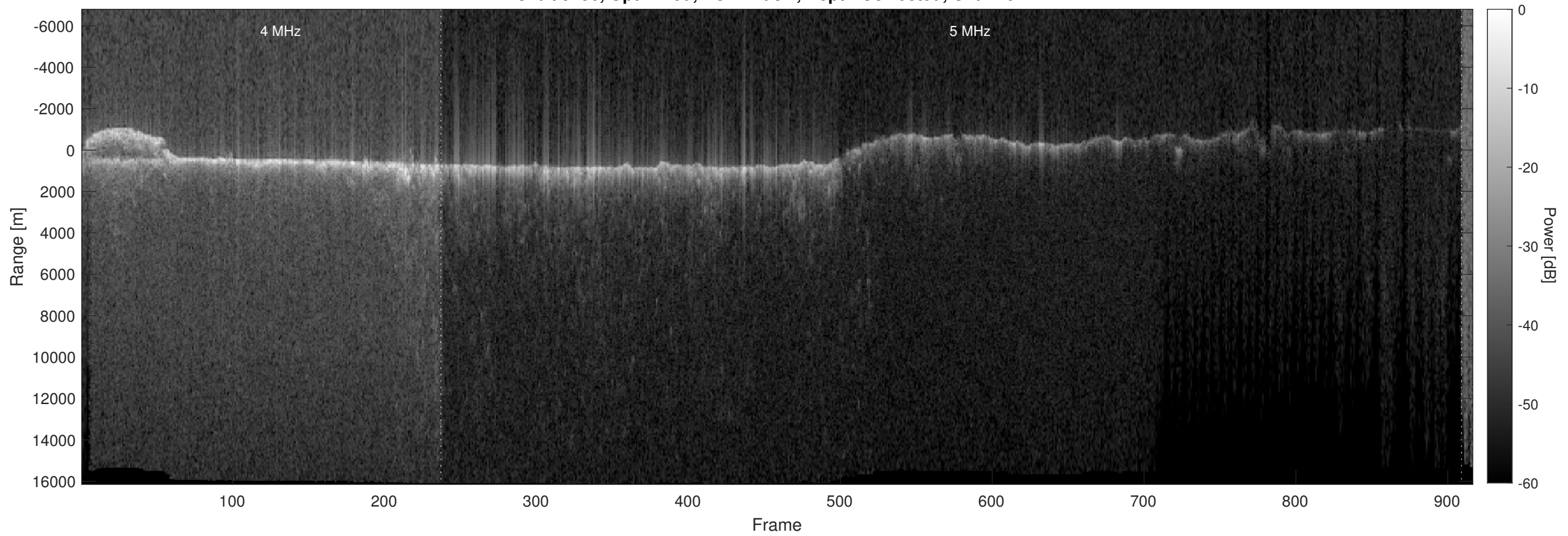
Orbit 9456, Optimized, No Window, Depth-Corrected, Channel 2
