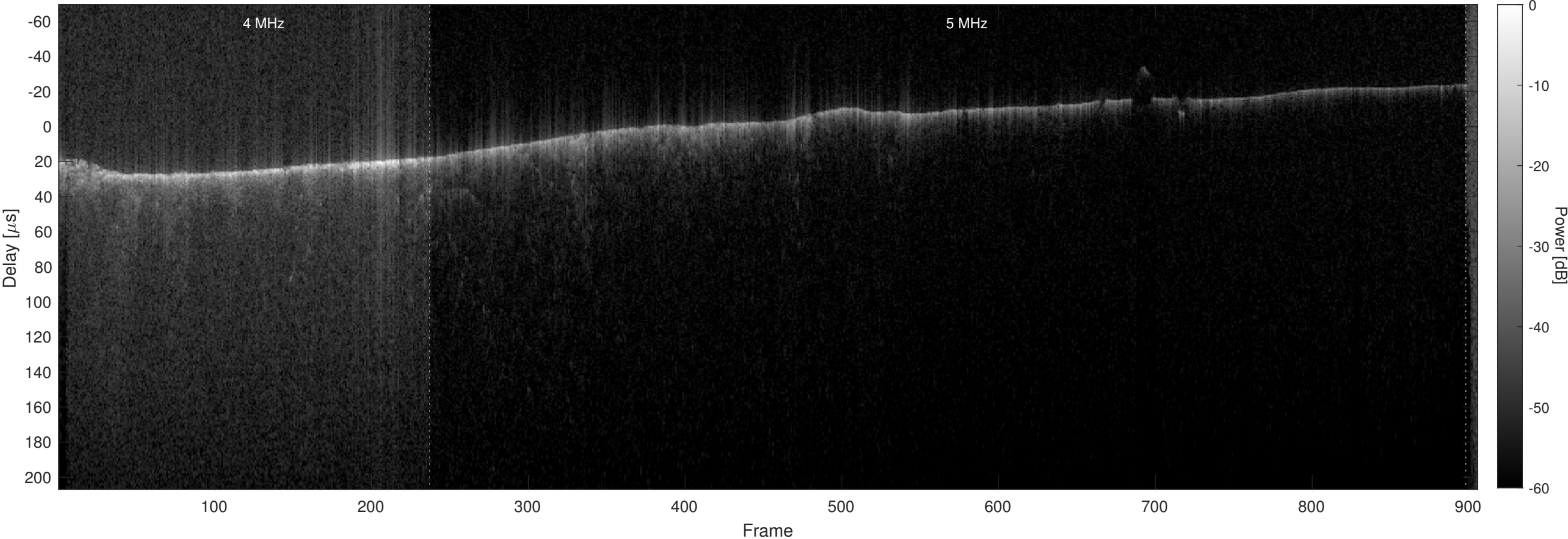
Orbit 9457, Optimized, No Window, Channel 2
