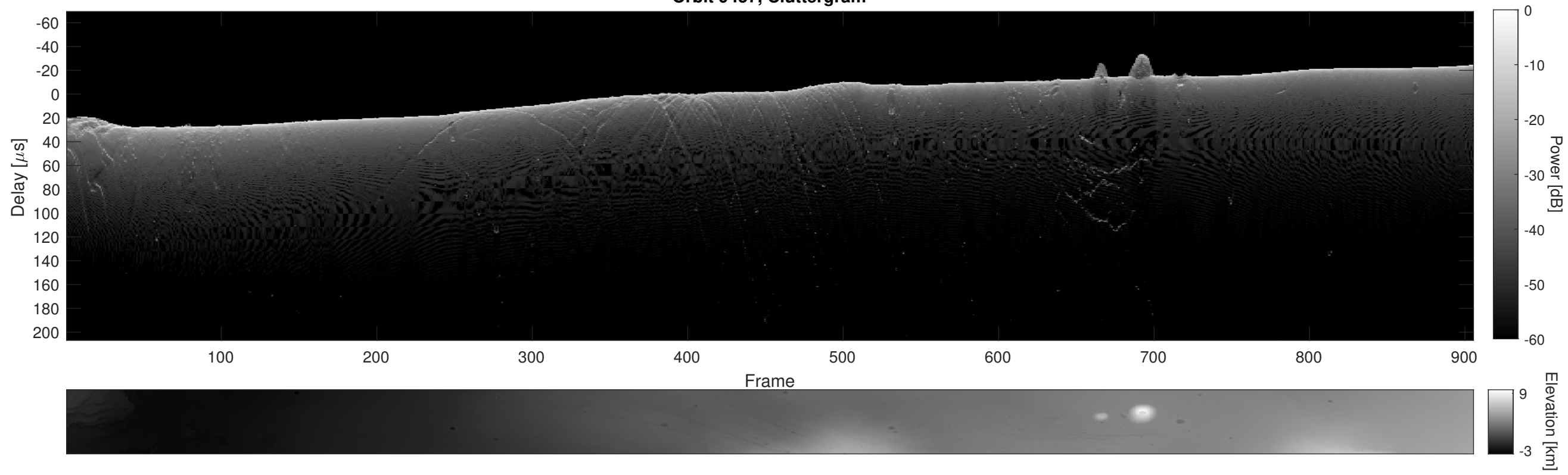
Orbit 9457, Cluttergram
