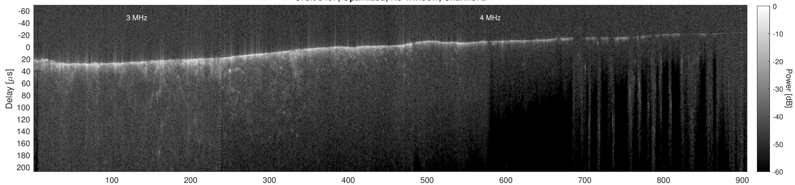
Orbit 9457, Cluttergram
