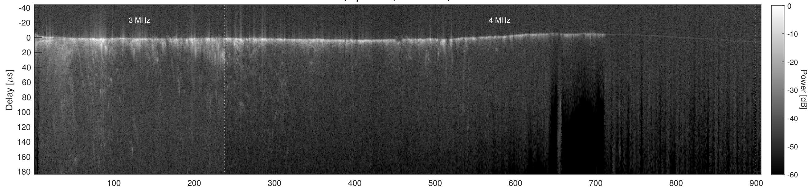
Orbit 9458, Cluttergram
