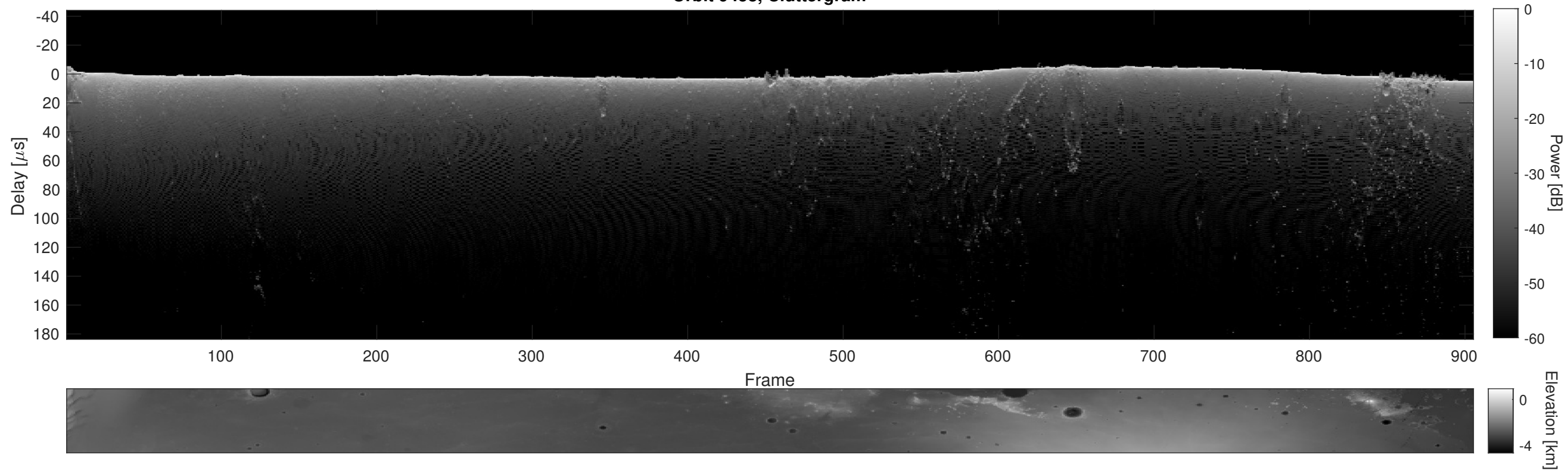
Orbit 9458, Cluttergram
