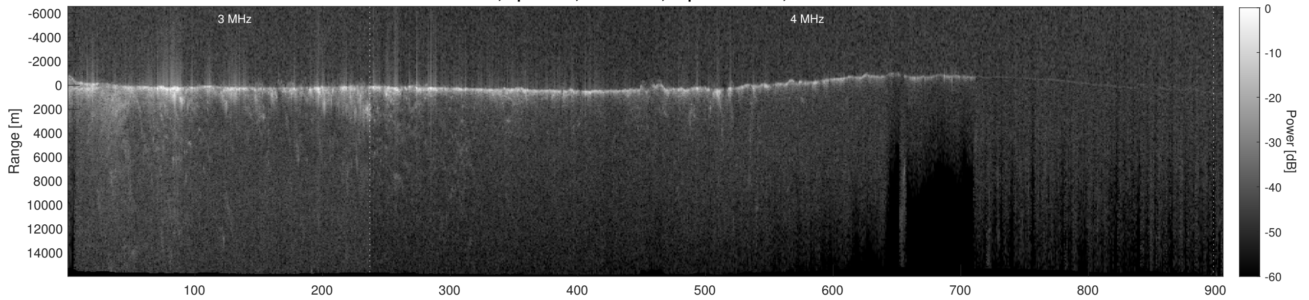
Orbit 9458, Depth-Corrected Cluttergram
