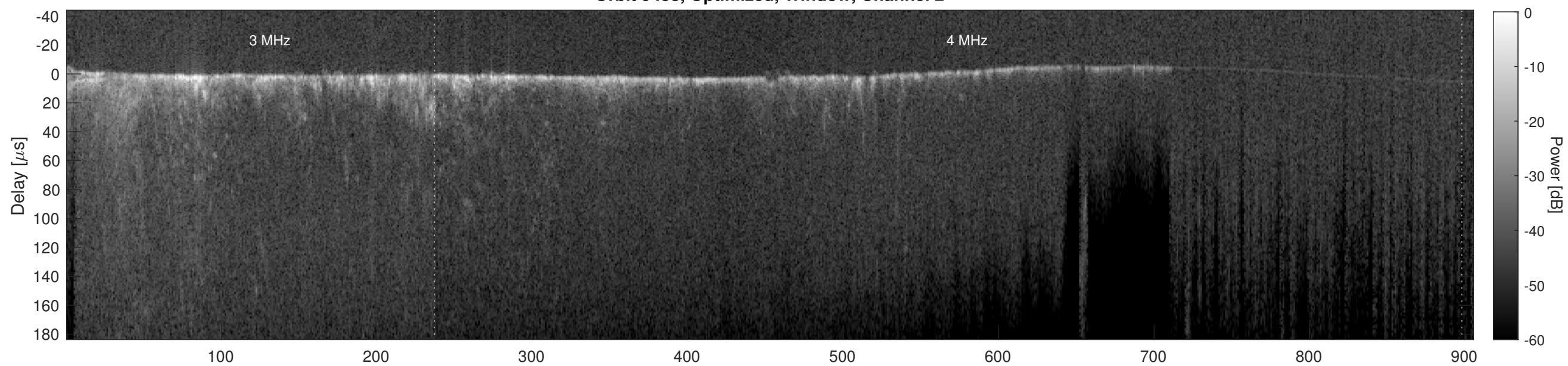
Orbit 9458, Cluttergram
