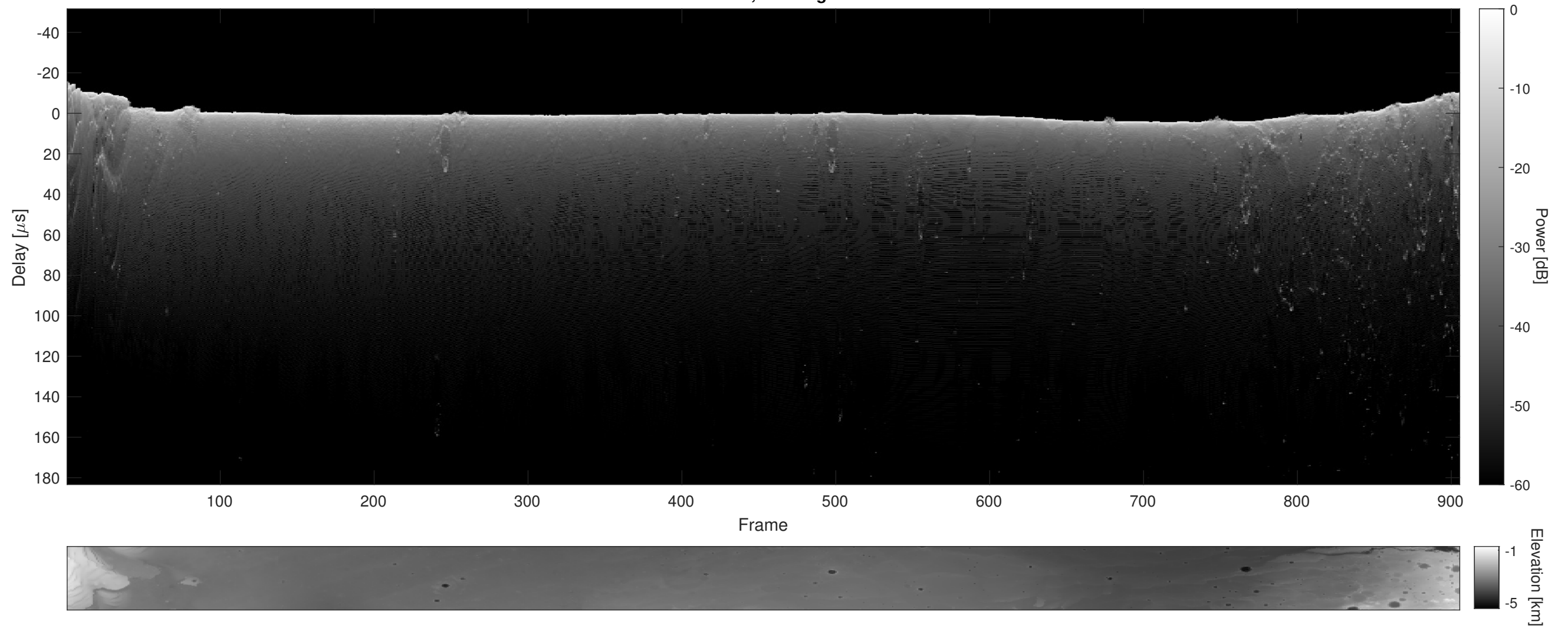
Orbit 9460, Cluttergram
