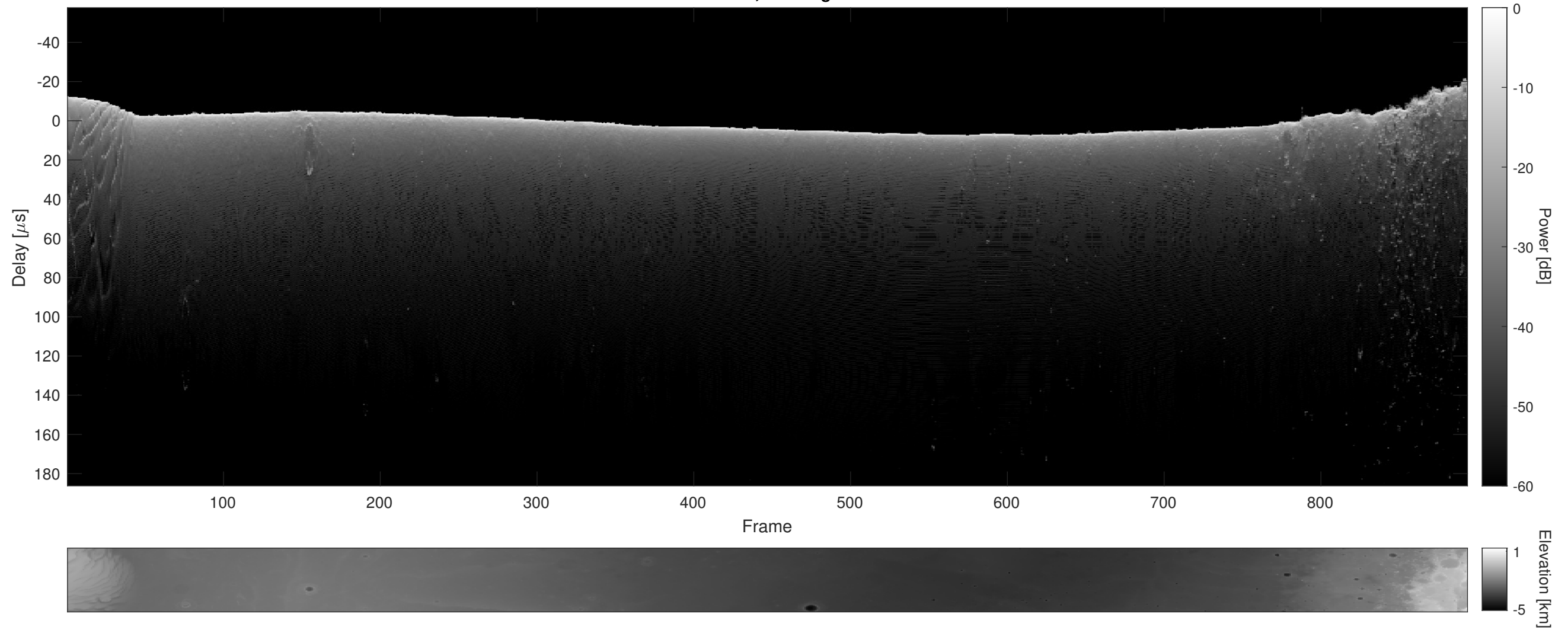
Orbit 9462, Cluttergram
