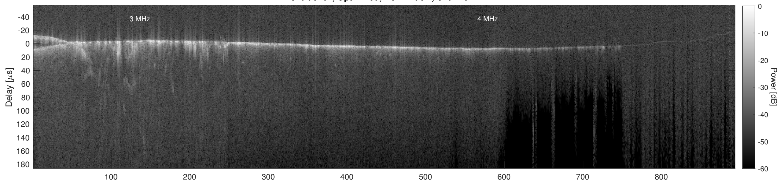
Orbit 9462, Cluttergram
