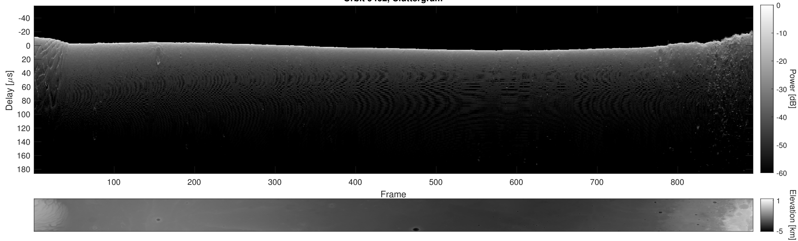
Orbit 9462, Cluttergram
