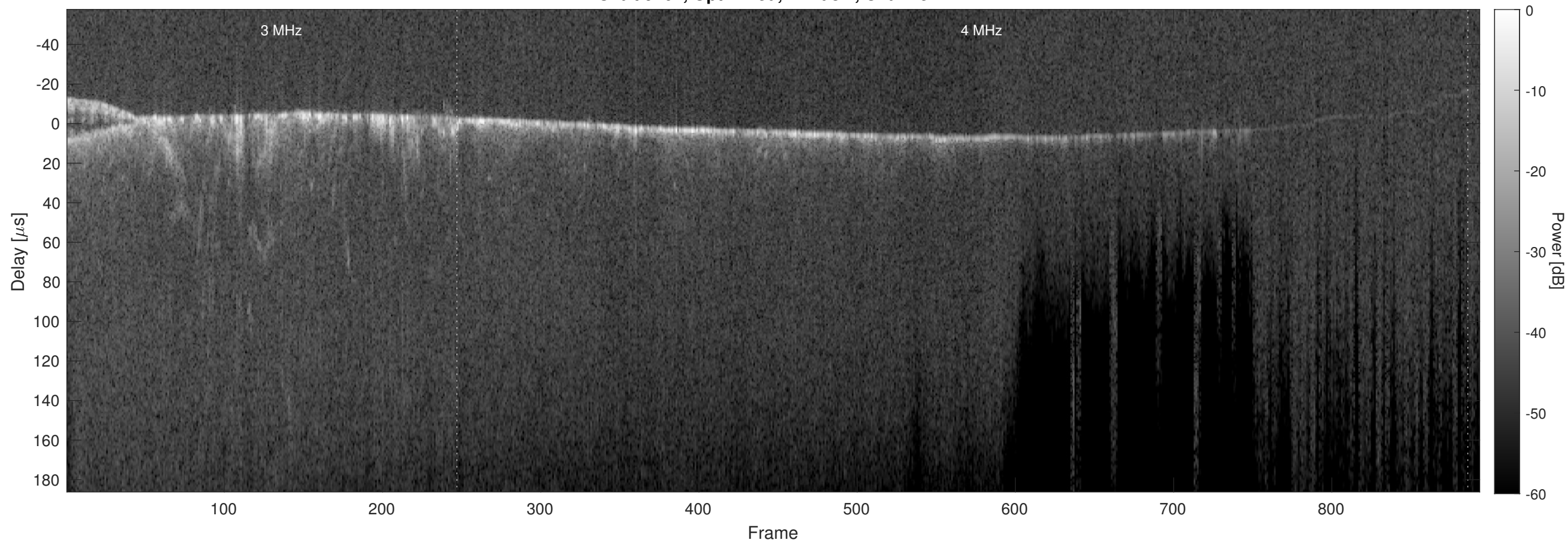
Orbit 9462, Optimized, Window, Channel 2
