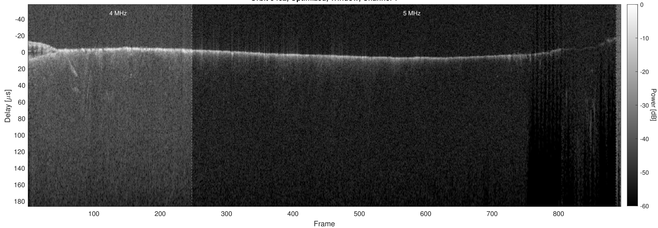
Orbit 9462, Optimized, Window, Channel 2
